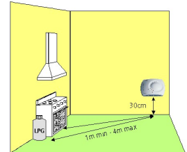
Fig.2: LPG gas detection
